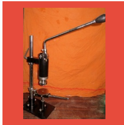
Perfume Bottle Crimping Machine
